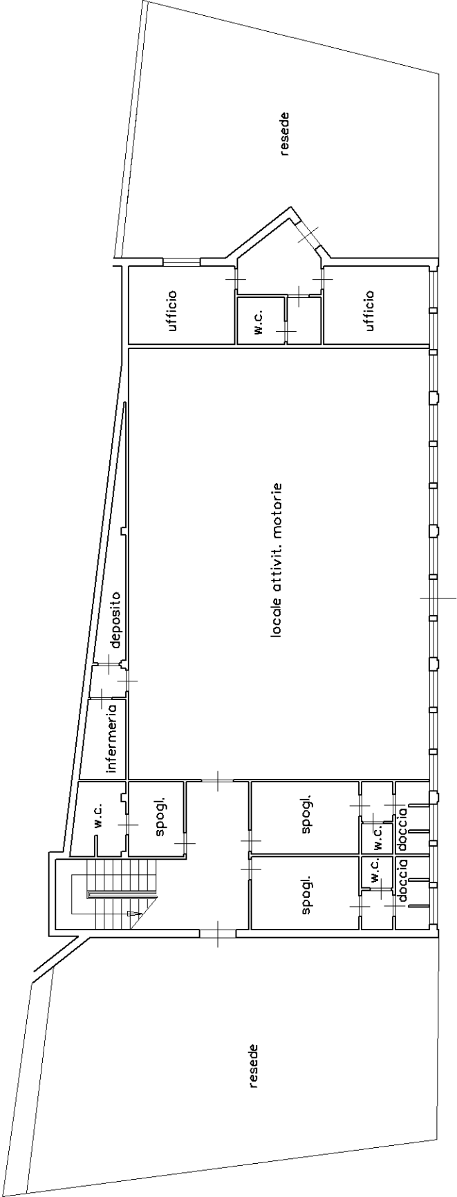
PIANO SEMINTERRATO H=4.50
